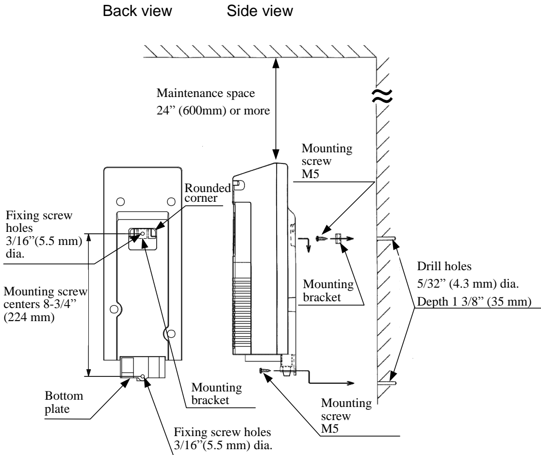
Fig.2-2 Installation of the equipment
