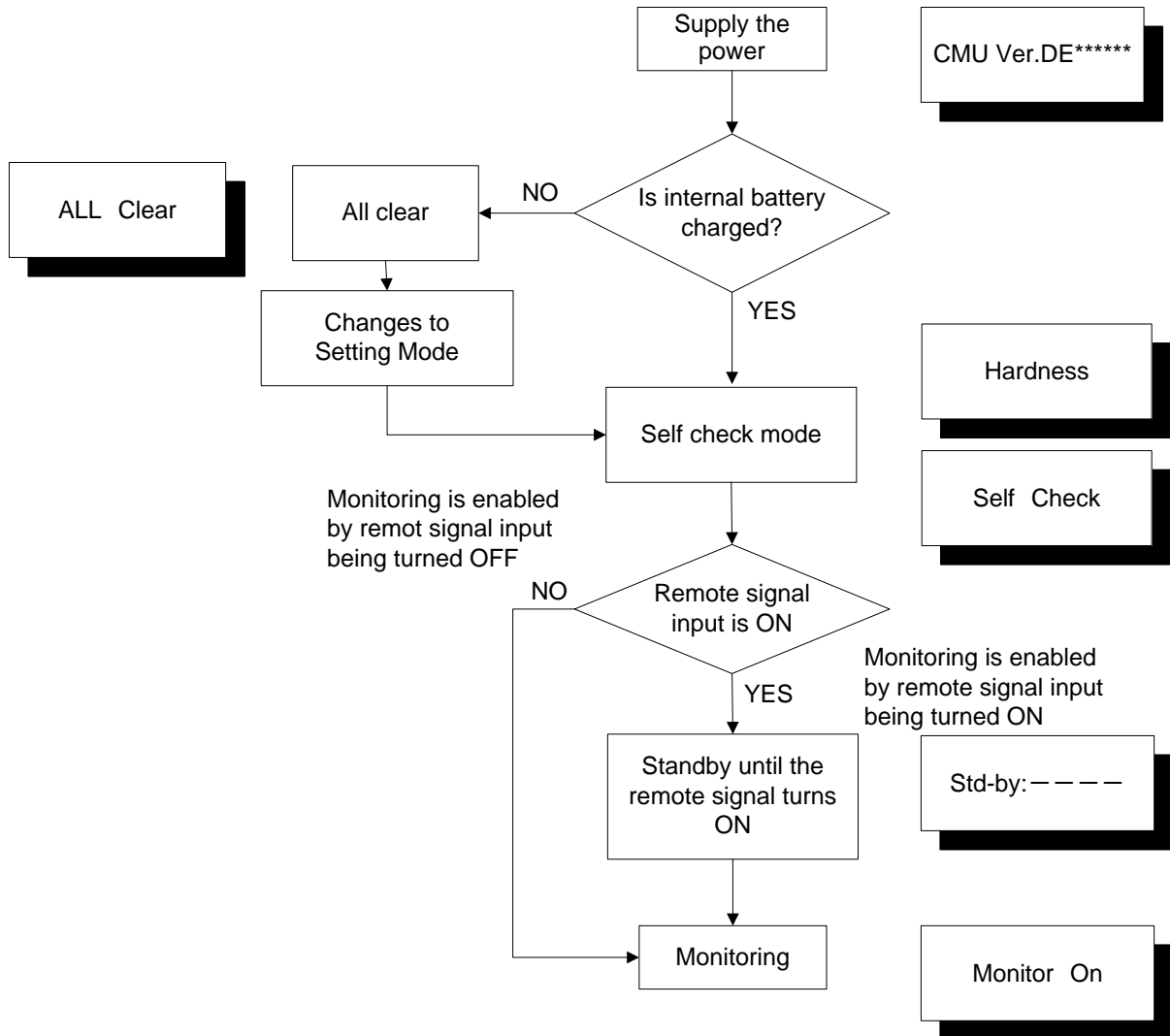
Flowchart of processes when the power supplied to the equipment
