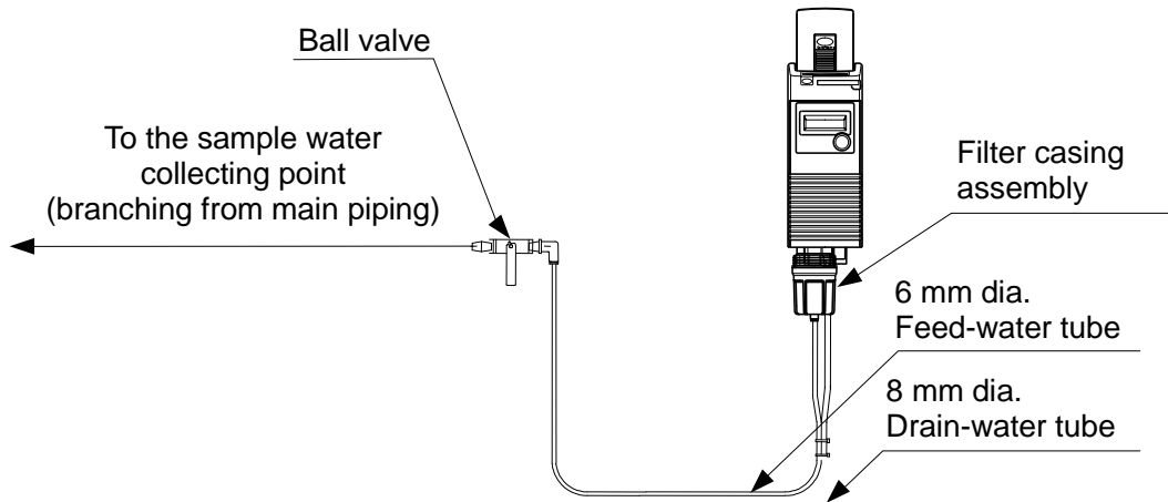
Fig3-1 Feed-water system
